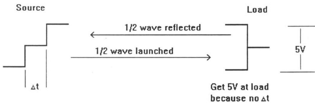
Fig. 2 Impedance Backmatching.
